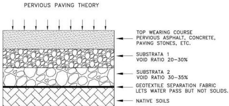
Figure 182. Pervious pavement detail ( https://www.grantspassoregon.gov/280/Pervious-Pavement-Alternative )
