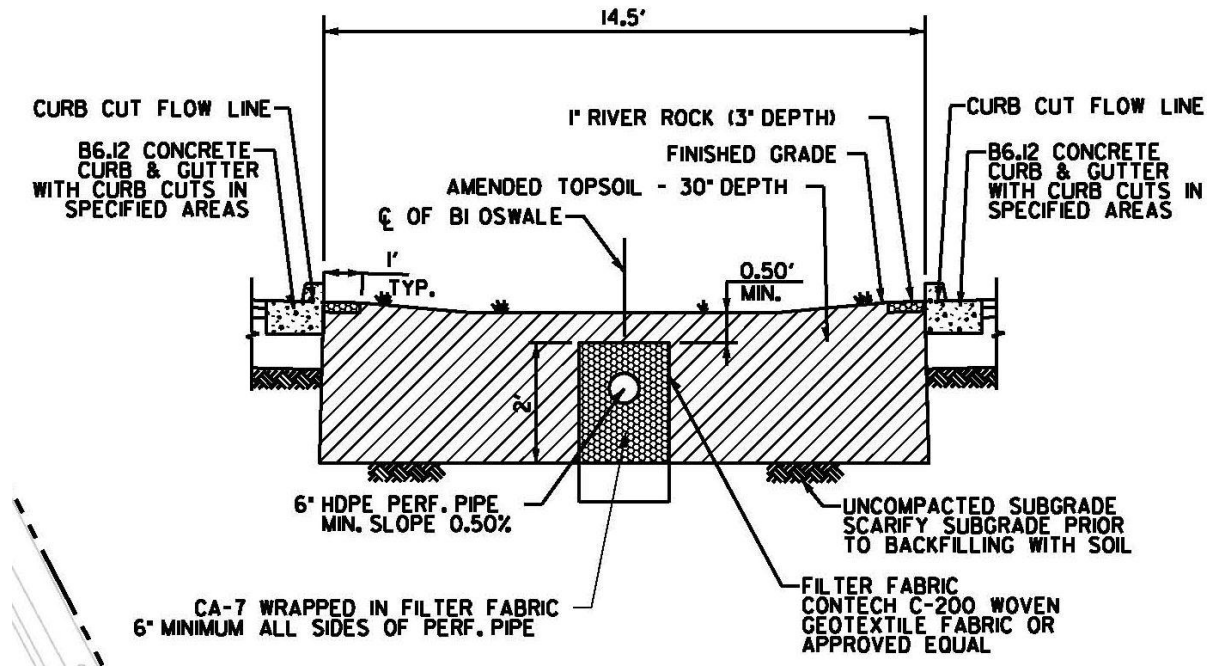
Figure 181. Construction detail of a bioswale ( https://www.warrenville.il.us/456/Bioswales )
