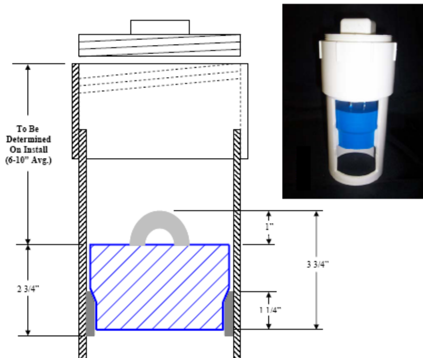
Figure 195. LDL plug design (Courtesy USSI)
