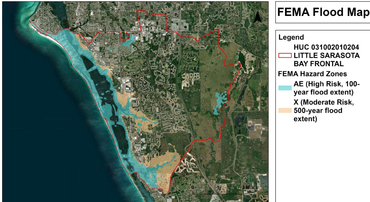
Figure 5. HUC 12 031002010204 Little Sarasota Bay Frontal FIRM map (2020), as generated by FAU CWR3.
