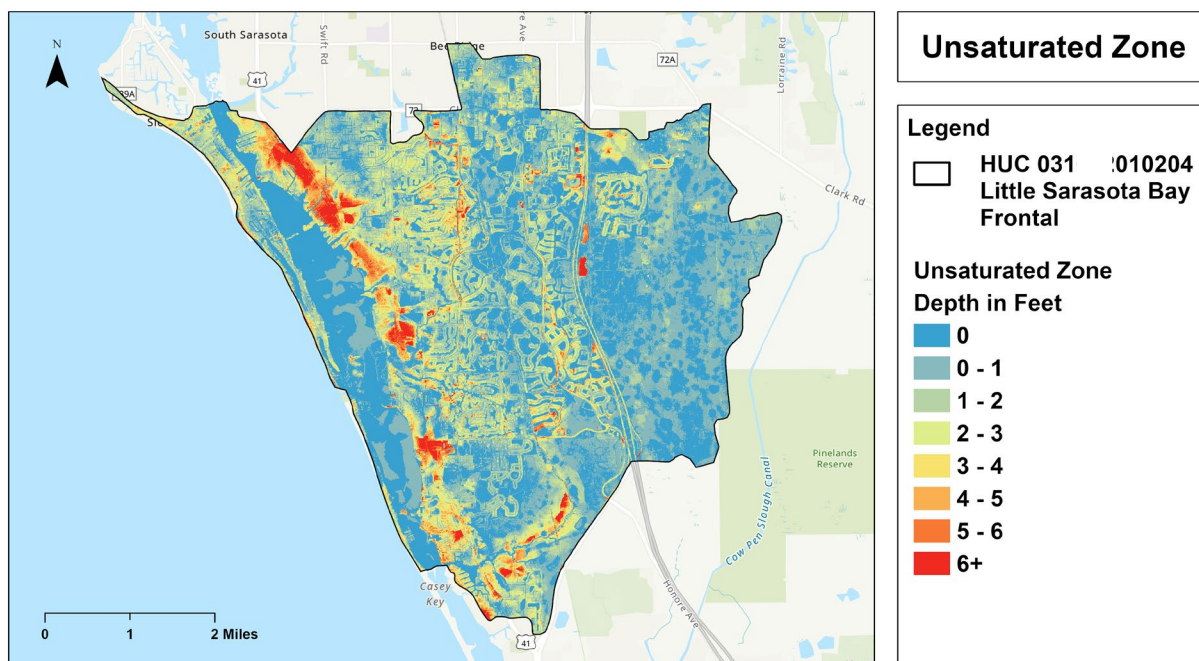
Figure 16. Unsaturated zone map for HUC 031002010204 Little Sarasota Bay Frontal, as generated by FAU CWR3.
