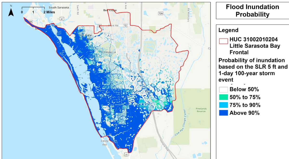
Figure 40. Probability of inundation based on 5 ft sea level rise and 1-day, 100-year storm for the HUC 031002010204 Little Sarasota Bay Frontal, as generated by FAU CWR3.
