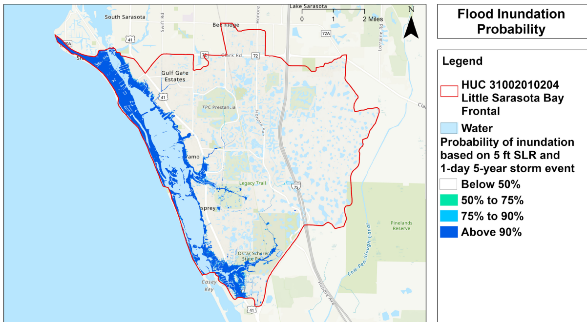
Figure 35. Probability of inundation based on 1-day, 5-year storm for the HUC 031002010204 Little Sarasota Bay Frontal, as generated by FAU CWR3.
