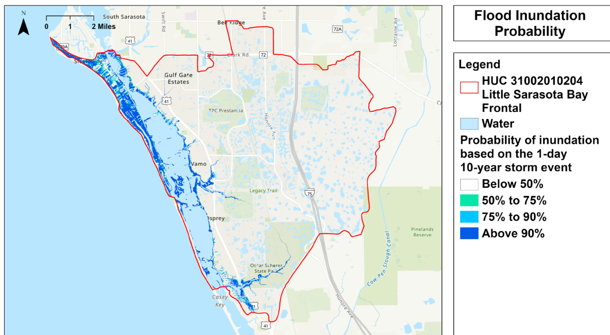
Figure 37. Probability of inundation based on 1-day, 10-year storm for the HUC 031002010204 Little Sarasota Bay Frontal, as generated by FAU CWR3.
