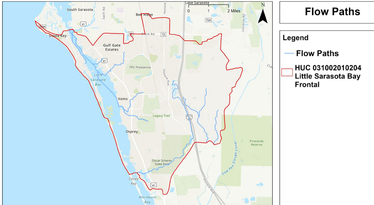
Figure 7. Flow paths for HUC 031002010204 Little Sarasota Bay Frontal sub-watershed (SWFWMD.gov), as generated by FAU CWR3.
